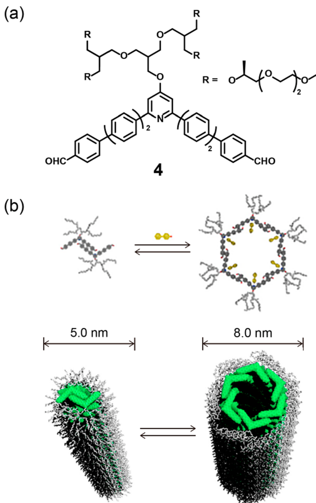
Figure 4. Reversible inflation of a self-assembled nanofiber into a hollow tubule. (a) Chemical structure of bent-shaped aromatic amphiphile 4 . (b) Schematic representation of the inflation process triggered by the guest. Reproduced with permission from ref 38. Copyright 2014 American Chemical Society.
