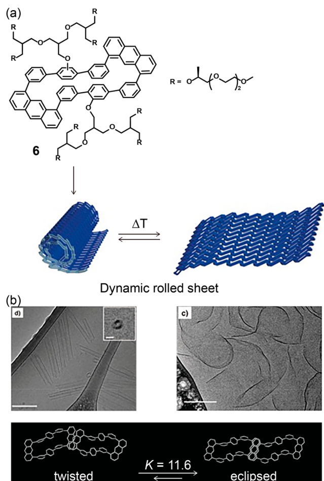
Figure 6. Dynamics rolling behaviors between scrolled tubules and flat sheets. (a) Chemical structure of aromatic amphiphile 6 . (b) Cryo-TEM images and molecular dynamics simulations of the reversible switching between folded and unfolded states (scale bar: 100 nm). Reproduced with permission from ref 26. Copyright 2016 Wiley.
