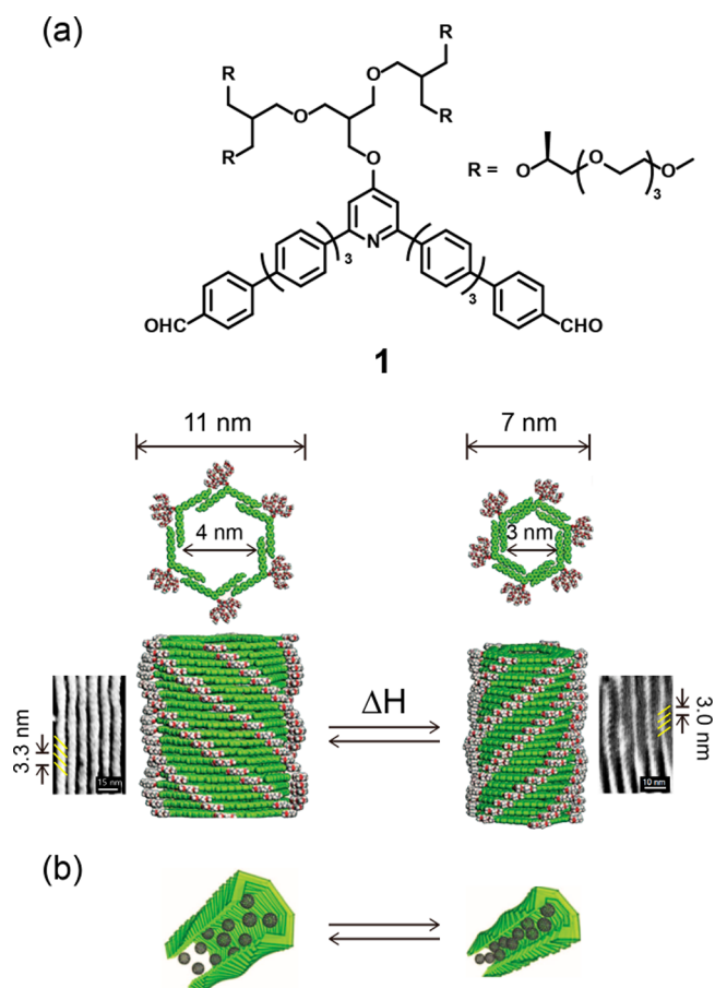
Figure 2. Reversible expanded–contracted switching of the tubular assembly with chirality inversion. (a) Chemical structure of bent-shaped aromatic amphiphile 1 . (b) Schematic representation of the expansion–contraction process with the chirality inversion and the regulated guest–guest interactions. Reproduced with permission from ref 25. Copyright 2012 The American Association for the Advancement of Science.
