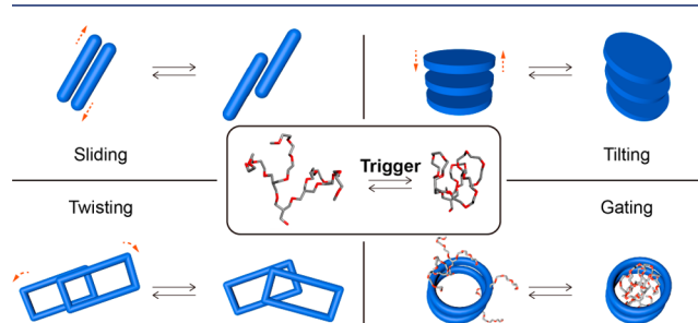
Figure 1. Representative switchable packing modes of aromatic segments triggered by phase transition of oligo(ethylene oxide) dendrons.
