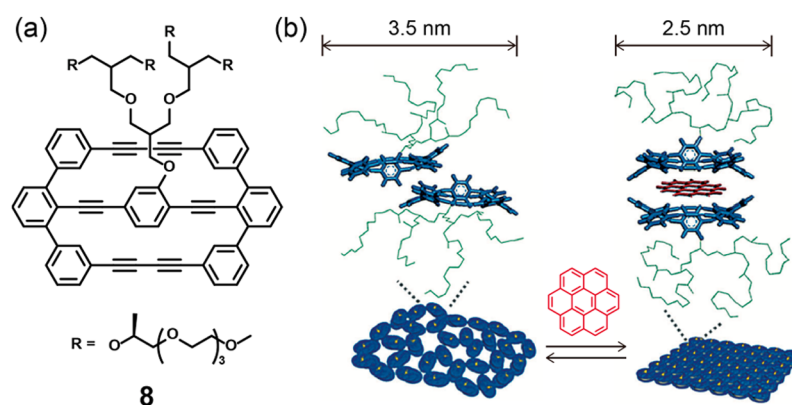
Figure 8. Dynamic motion of 2D porous sheets between open and closed states. (a) Chemical structure of aromatic amphiphile 8 . (b) Schematic representation of the switch between a nanoporous sheet and a closed sheet triggered by guest intercalation. Reproduced with permission from ref 54. Copyright 2013 Wiley.
