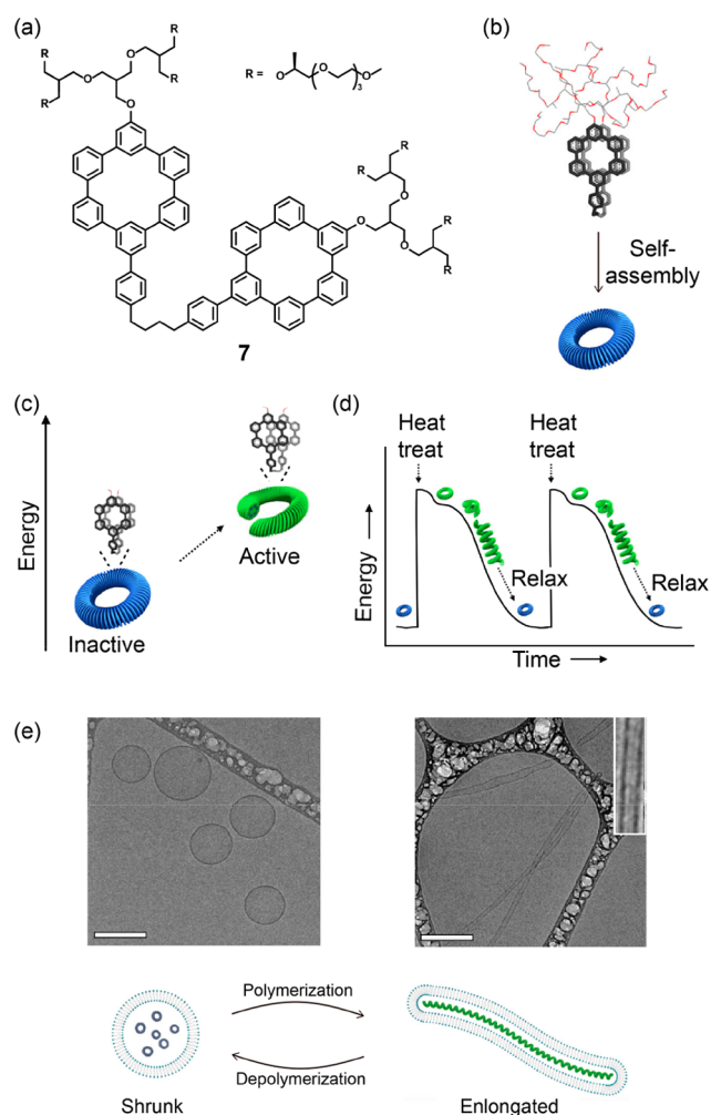
Figure 7. Heat-fueled dissipative helical assembled polymers. (a) Chemical structure of macrocycle dimeric amphiphile 7 . (b) Schematic representation of the toroidal assembly through an eclipsed conformation. (c) Tilting transition of the toroids active by heat. (d) Energy landscape of polymerization/depolymerization cycles. (e) Cryo-TEM images and schematic representation of the elongated-contracted motion of the vesicle with the toroids inside by spontaneous polymerization/depolymerization (scale bar: 200 nm). Reproduced with permission from ref 1. Copyright 2019 Springer Nature.
