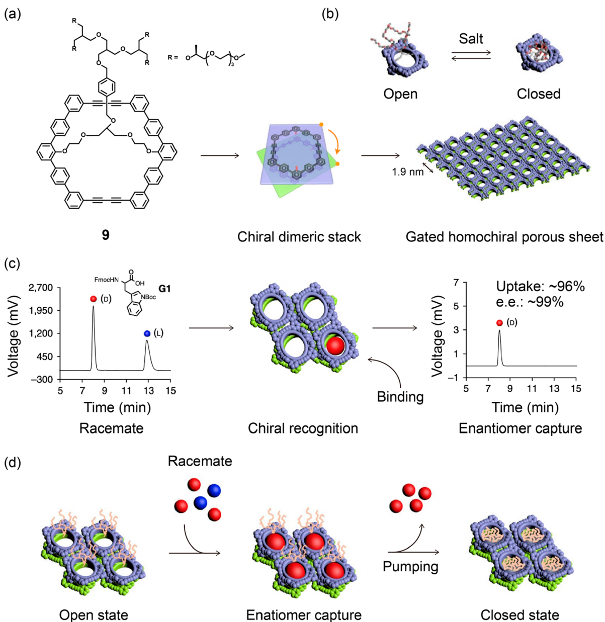
Figure 9. Open–closed gating of homochiral porous nanosheets for enantiomer sieving. (a) Chemical structure of aromatic macrocycles 9 and schematic representation of the formation of homochiral porous nanosheets. (b) Open–closed gating behavior triggered by salt. (c) Chiral recognition and macroscopic separation. (d) Chiral recognition, enantiomer sieving, and pumping action by addition of salt. Reproduced with permission from ref 2. Copyright 2018 Springer Nature.
