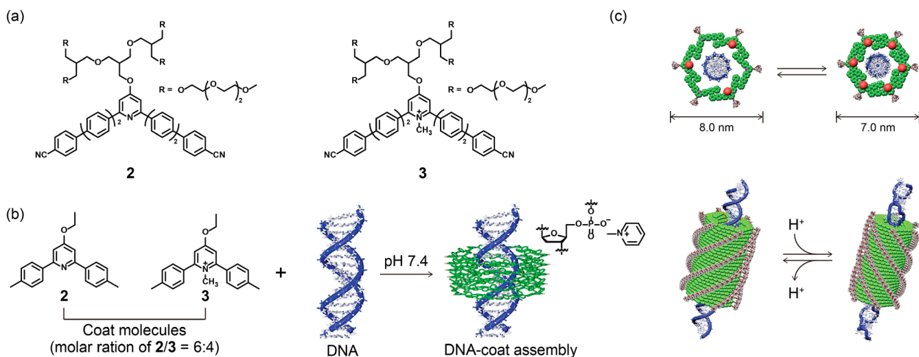
Figure 3. Collective helicity switching of the DNA–coat assembly. (a) Chemical structure of coat molecules 2 and 3 . (b) Schematic representation of the interactions between coat molecules and DNA to form the assembly at pH 7.4. (c) Schematic representation of the collective motion of the DNA–coat assembly with a helicity inversion by a pH change. Reproduced with permission from ref 3. Copyright 2017 Springer Nature.
