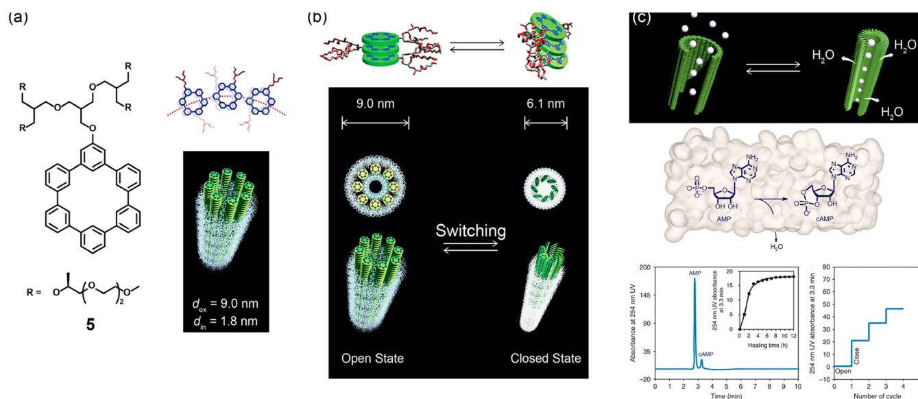
Figure 5. Open–closed gating of the tubular pores. (a) Chemical structure of disc-shaped aromatic amphiphile 5 . (b) Schematic representation of the open–closed switching caused by the slipped aromatic packing triggered by heat. (c) Dehydrative cyclization of AMP to yield cAMP in the closed tubule by water pumping action. Reproduced with permission from ref 4. Copyright 2015 Springer Nature.
